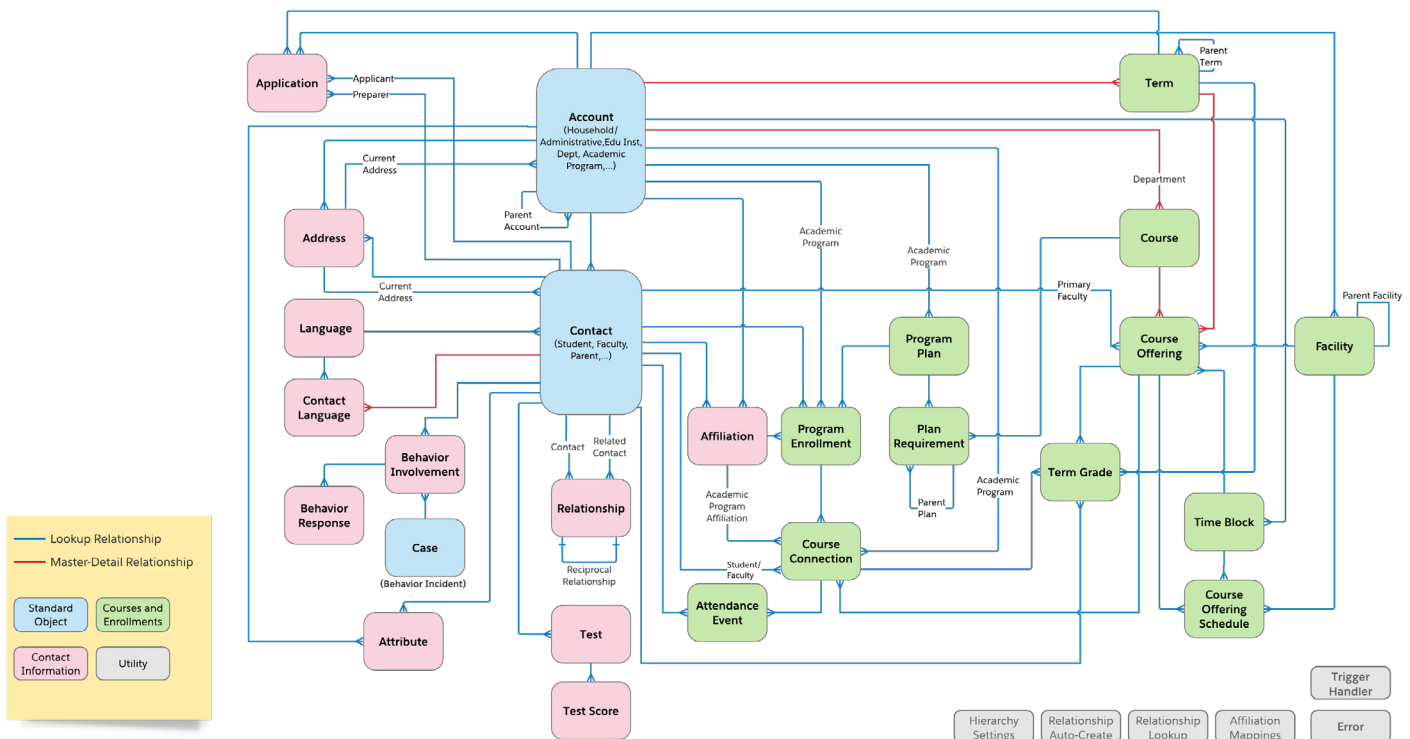
An Entity-Relationship Diagram (ERD) showing how EDA works with each database object and their relationships
